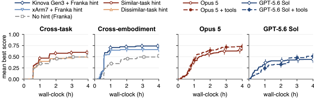
Figure 6: Evaluations on cross-task and cross-embodiment transfer (left two) and with additional tools (right two). Markers with vertical bars at hourly intervals show mean \pm SEM across runs (2 models \times 3 seeds per task for the generalization runs; one run per task for the tool runs).
