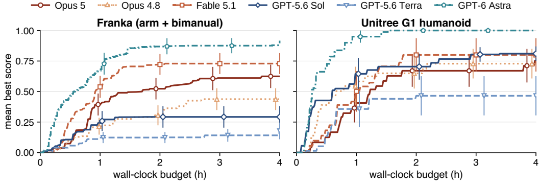
Figure 15: Best-so-far score versus wall-clock time, by embodiment.
