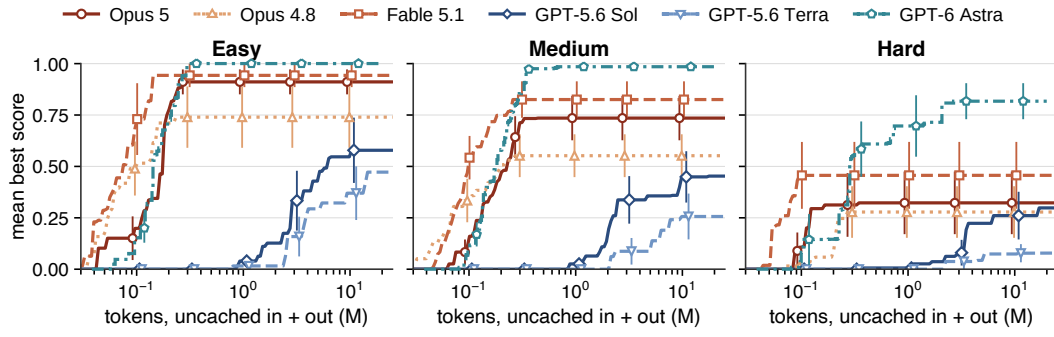
Figure 12: Best-so-far score versus generated tokens, by difficulty tier.
