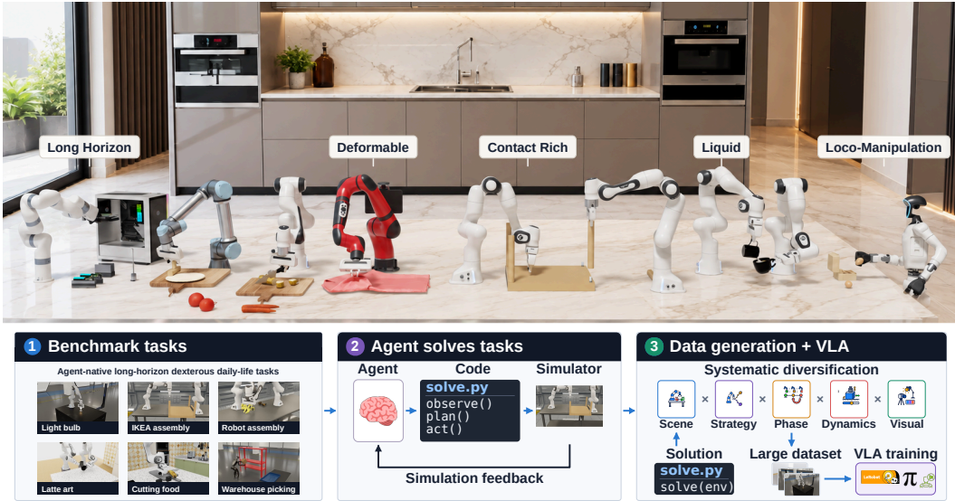
Figure 1: Overview of our framework: Top : EMBODIEDSWE-BENCH contains diverse long-horizon robotics tasks. Bottom : coding agents solve these tasks and turn verified solutions into scalable supervision for general policies.
