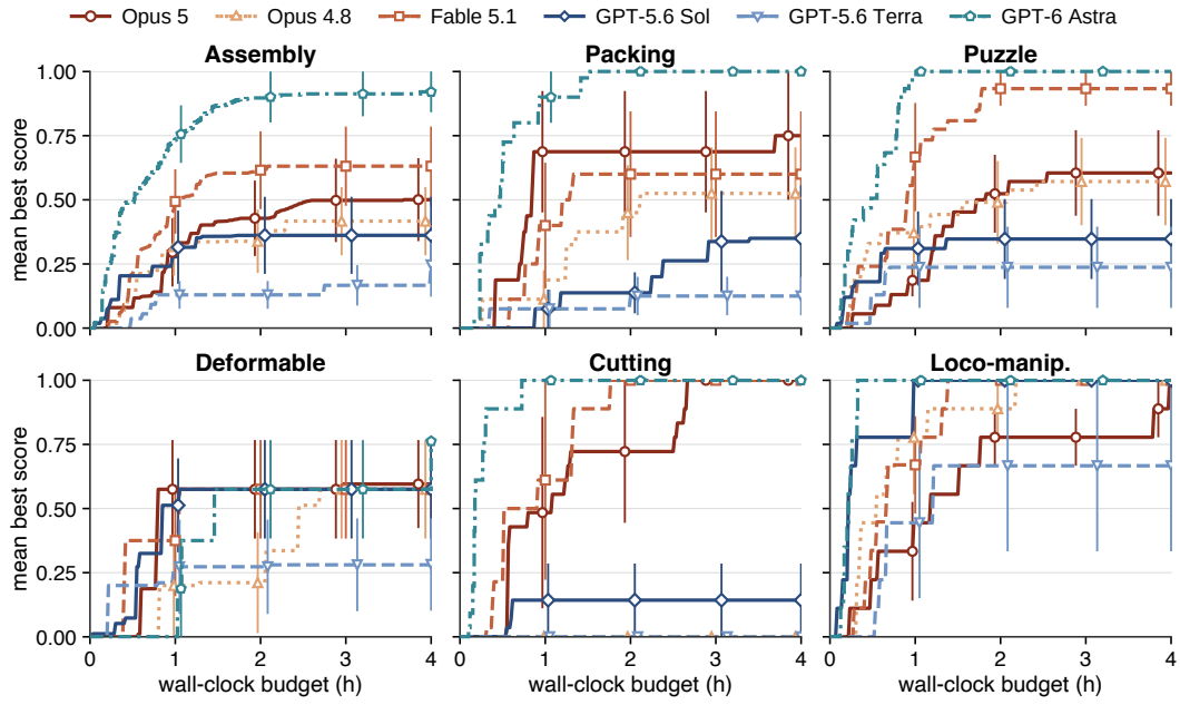
Figure 13: Best-so-far score versus wall-clock time, by suite.
