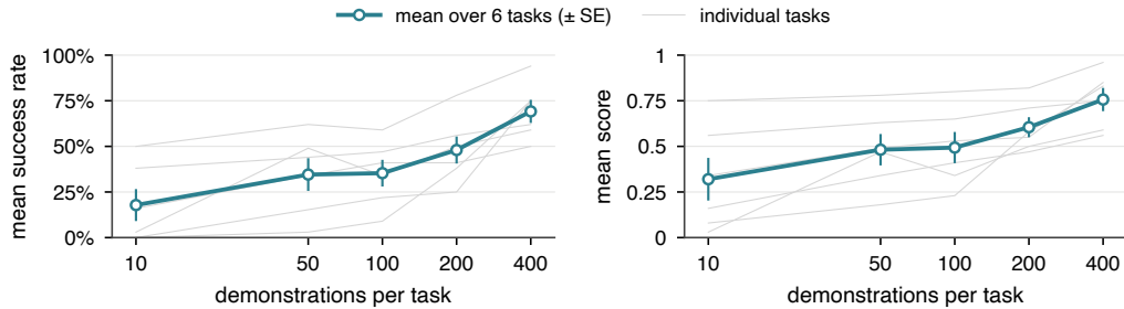
Figure 9: VLA finetuning with generated in-distribution demonstrations. Mean task scores and success rates at five training-set sizes. Overall performance improves as more generated demonstrations are provided.
