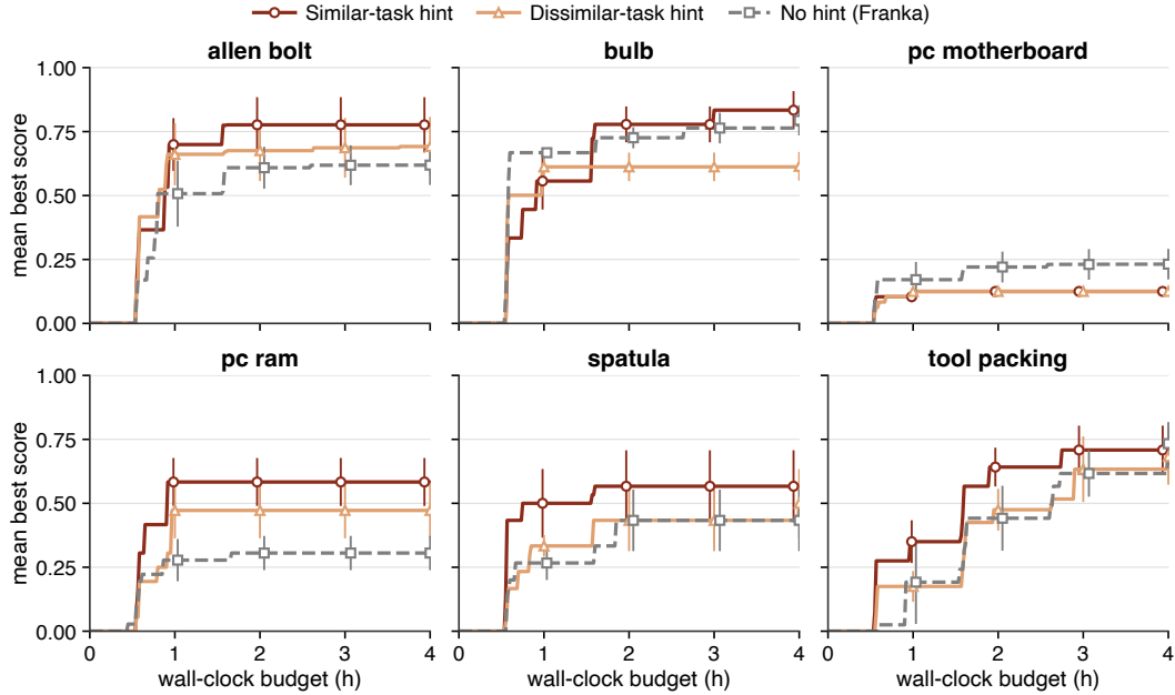
Figure 17: Cross-task generalization by target task. Rubric score versus agent wall-clock time (mean \pm SEM over 2 models \times 3 seeds) for the similar-task hint, dissimilar-task hint, and no-hint settings.
