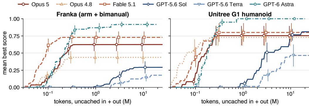
Figure 16: Best-so-far score versus generated tokens, by embodiment.
