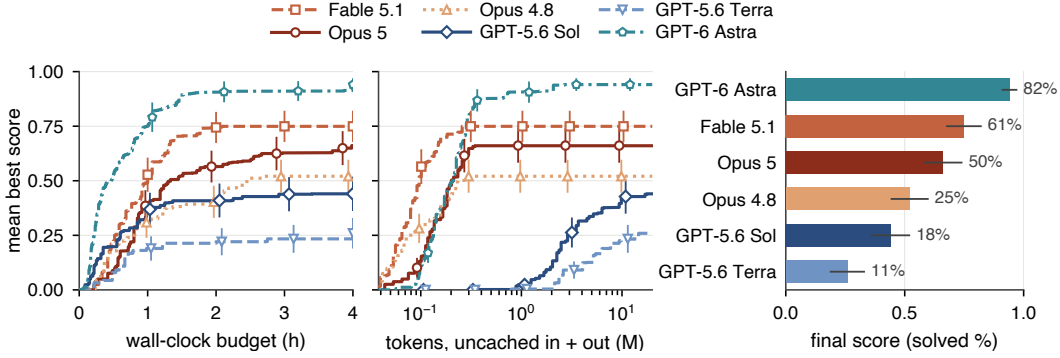
Figure 3: Base results on EMBODIEDSWE-BENCH. Left, middle: mean best-so-far score over 28 tasks against wall-clock and tokens; markers with vertical bars at hourly intervals / fixed token counts show mean \pm SEM across tasks (one run per task). Right: mean final score with SEM across tasks; percentages give the fraction of tasks solved.
