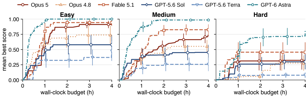
Figure 11: Best-so-far score versus wall-clock time, by difficulty tier.
