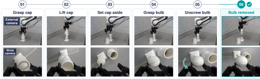
Figure 10: Successful real-robot lamp disassembly rollout from a policy finetuned only on coding-agent-generated simulation data
