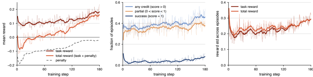
Figure 20: RL training curves.
