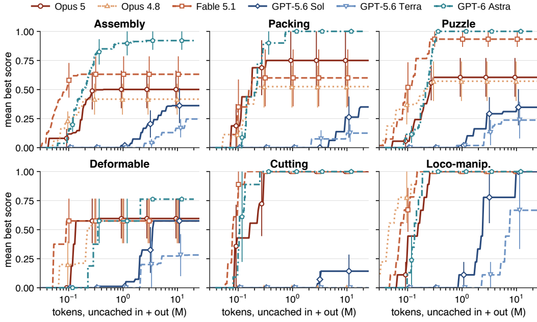
Figure 14: Best-so-far score versus generated tokens, by suite.
