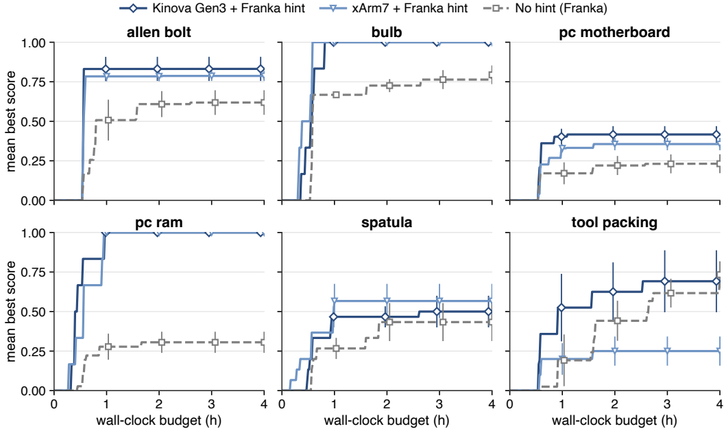
Figure 18: Cross-embodiment generalization by task. Rubric score versus agent wall-clock time (mean \pm SEM over 2 models \times 3 seeds) for the two target embodiments given the Franka reference solution as a hint. From-scratch Franka runs are shown as a reference for task difficulty.
