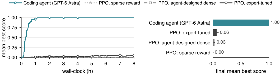
Figure 5: Programmatic policies versus RL. Despite stronger supervision and extensive tuning, RL substantially underperforms coding-agent policies.
