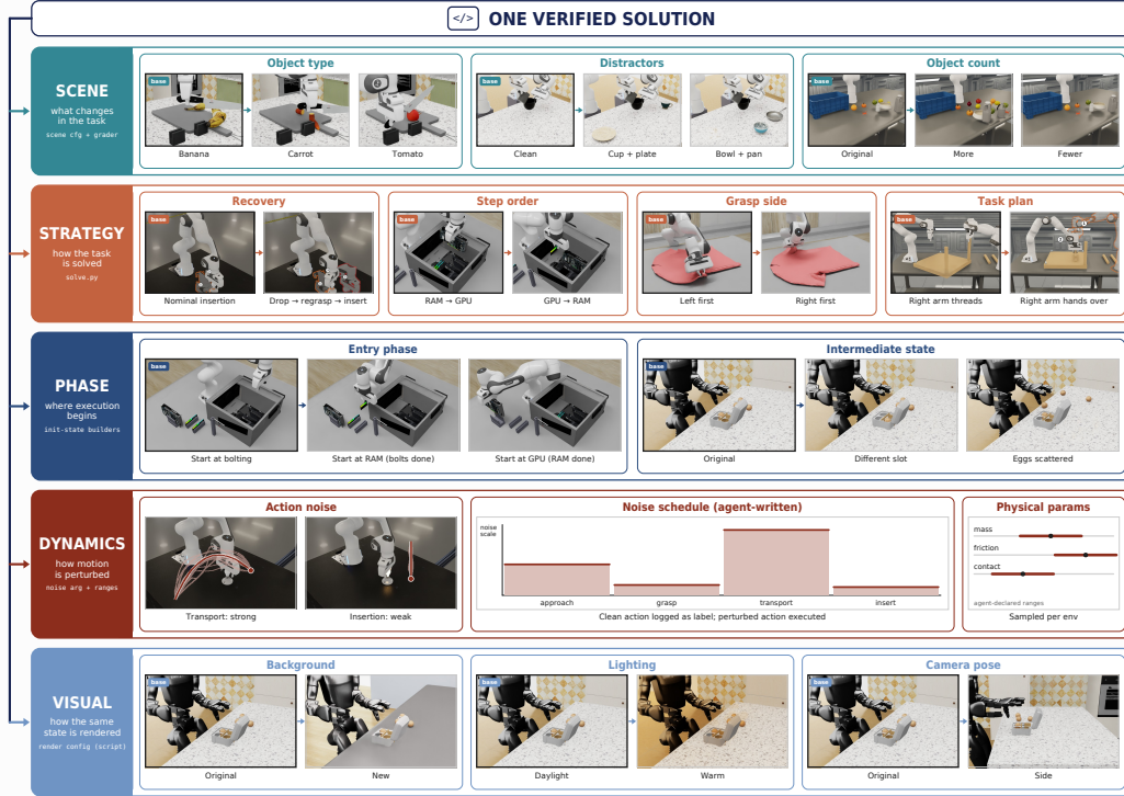
Figure 7: Hierarchical diversification pipeline of EMBODIEDSWE-GEN. Starting from one verified coding-agent solution, we diversify the scene , strategy , phase , dynamics , and visual to expand it into a broad set of training trajectories. Higher-level variations modify task structure, solution behavior, and intermediate-state coverage, while lower-level variations introduce physical, action, and visual perturbations to improve robustness and diversify execution.
