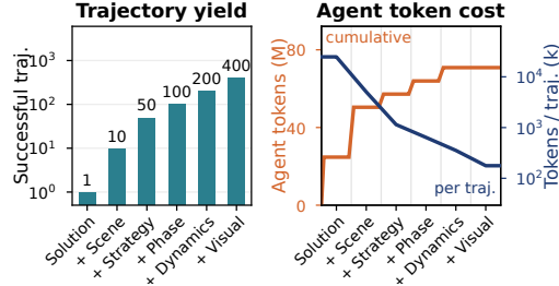
Figure 8: One verified solution can be expanded into many diverse trajectories through hierarchical diversification, with only modest additional agent cost per variation and rapidly decreasing amortized cost at scale.
