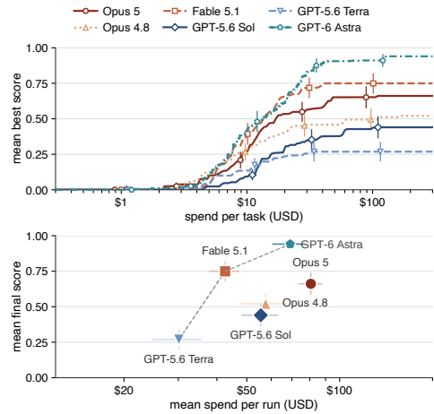
Figure 4: Score against cost.
